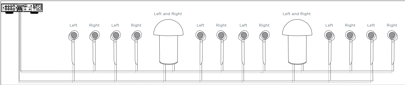
SONARRAY 12:2 CONFIGURATION
