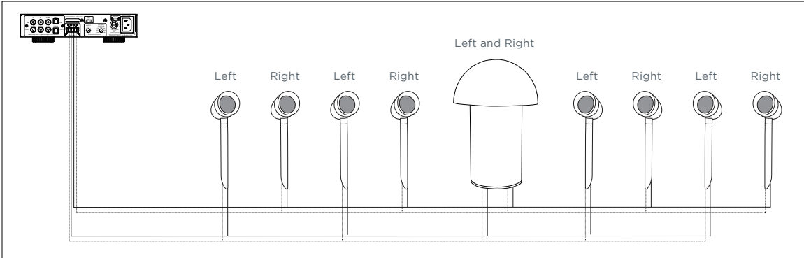
SONARRAY 8:1 CONFIGURATION
